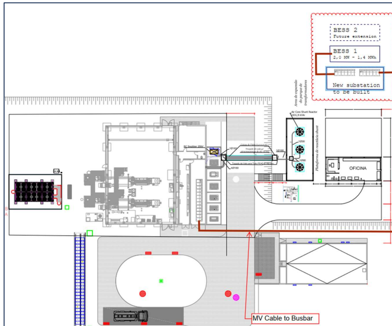
Figure 4 – ESS Location and Outcoming Feeder to the Electra power plant (Santo Antão)
