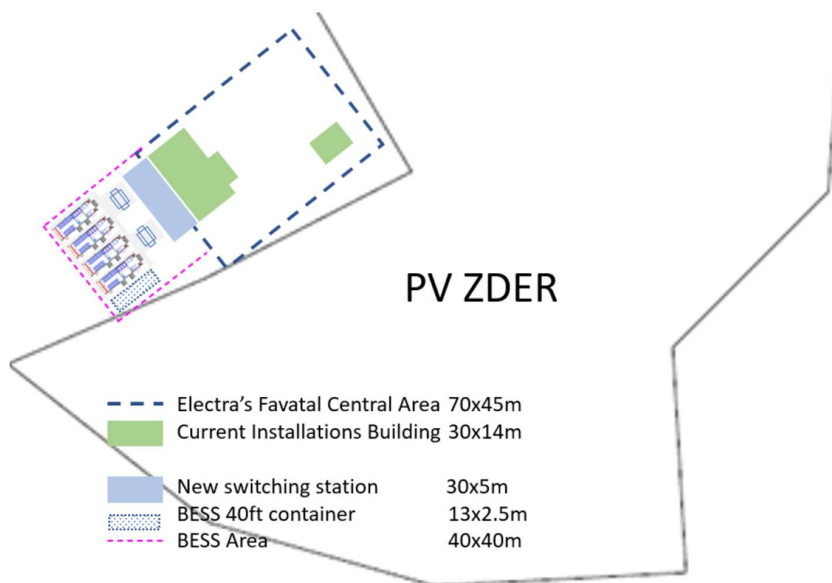
Figure 10 - ESS Location and Outcoming Feeder to the Electra power plant (Brava)
